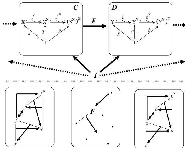
Figure 6: Coupling of Completely Closed Systems in the Different Categories and the Hyperdigraphs
